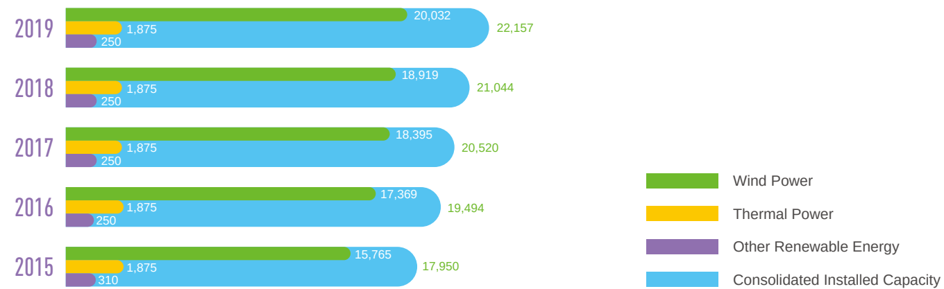
Total Installed Capacity in the Last Five Years Unit: MW
